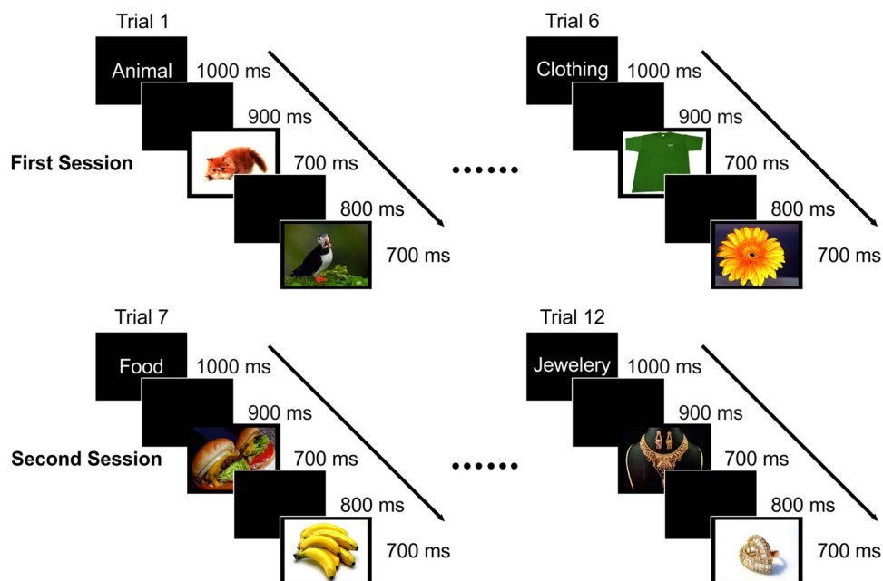
Fig. 1 “Cued-target” with “go/no-go” task paradigm. Target cue remained on the screen for 1 s, after an additional 900 ms delay, the images were presented. Each image was presented for 700 ms with 800 ms interval time between two images and 5 s black screen for rest between two different categories
